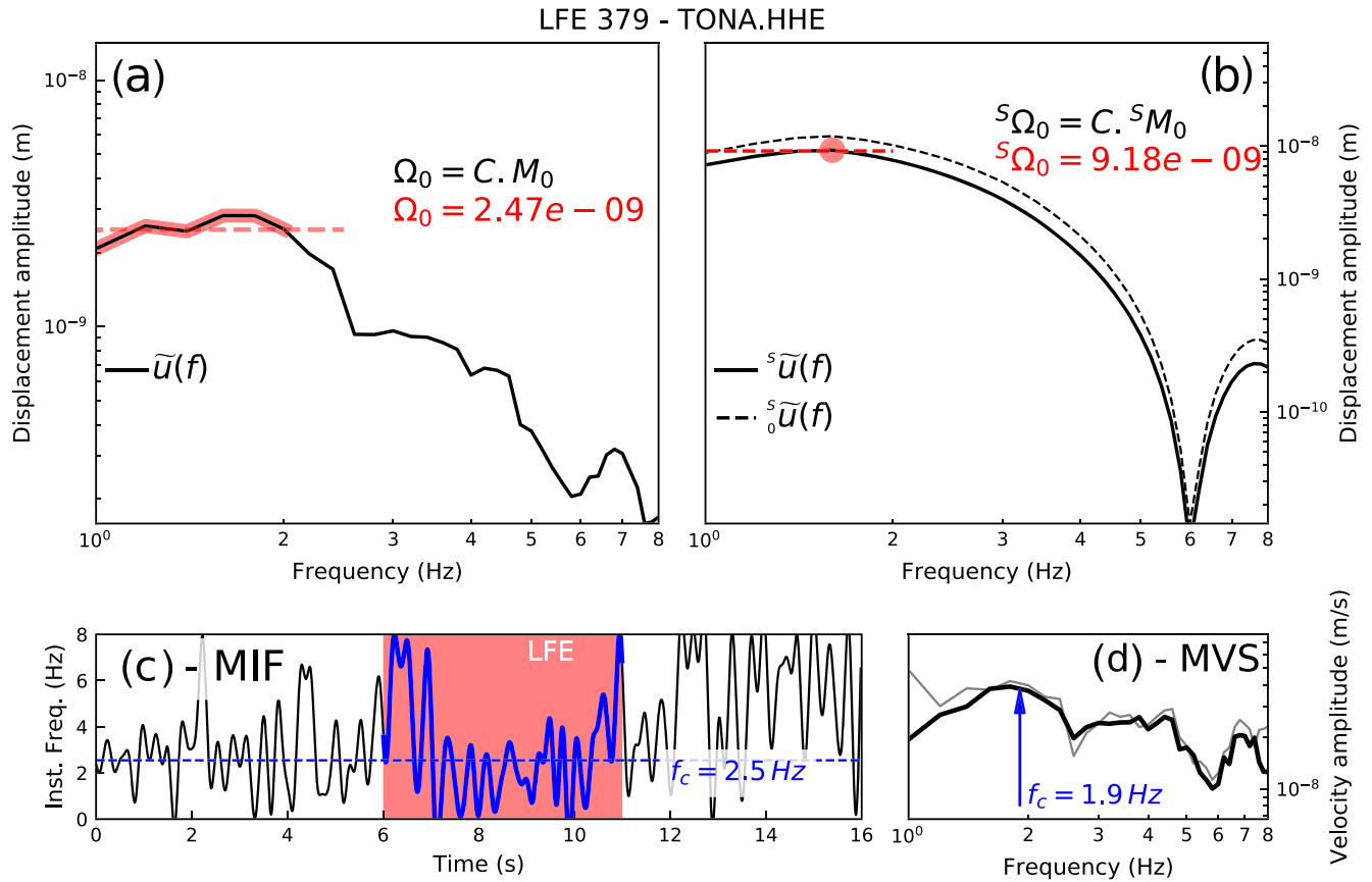
Figure 4. Determination of the seismic moment M_0 and corner frequency f_c for an example low-frequency earthquake. Example LFE: nb. 379, Channel HHE of Station TONA. (a) \Omega_0 is determined as the red plateau of the displacement spectrum. (b) {}^S\Omega_0 is determined as the maximum of the synthetic displacement spectrum, taking into account attenuation. (c) The corner frequency f_c is measured as the mean instantaneous frequency (MIF) over the waveform time window (see Figure 3 for the LFE waveforms) (d) and as the maximum of the velocity spectrum (MVS) of the waveform. In gray, the unfiltered velocity spectrum, allowing to assess the effects of the 1–8 Hz filter on the spectrum.
