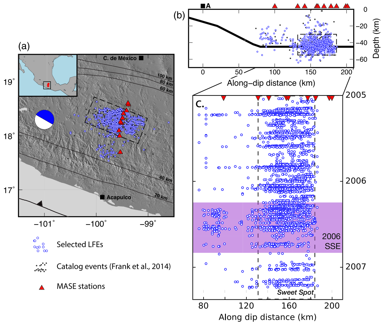
Figure 1. Spatial and temporal distribution of the selected LFEs. (a and b) Selected LFEs are plotted as white and blue dots, and the bulk catalog of (Frank et al., 2014) is in gray. Subduction interface depth contours are displayed in black (Kim et al., 2010). The focal mechanism corresponds to an average mechanism computed from cataloged LFE detections (Frank et al., 2013). (c) The time-dip distribution of the events.
