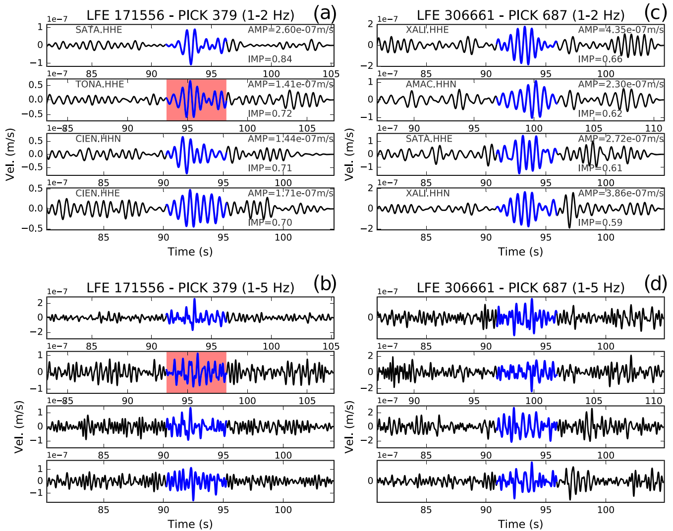
Figure 3. Selected LFEs' waveforms. The four most impulsive waveforms of LFE 379 and 687 are displayed here, 1–2 Hz band-pass filtered (a and c) and between 1 and 5 Hz (b and d). The blue section of the waveform shows the time window used to define the detected signal, and the red patch shows which channel's waveforms are used as an example for source parameters characterization in Figure 4. Impulsivity and amplitude are indicated for each channel.
