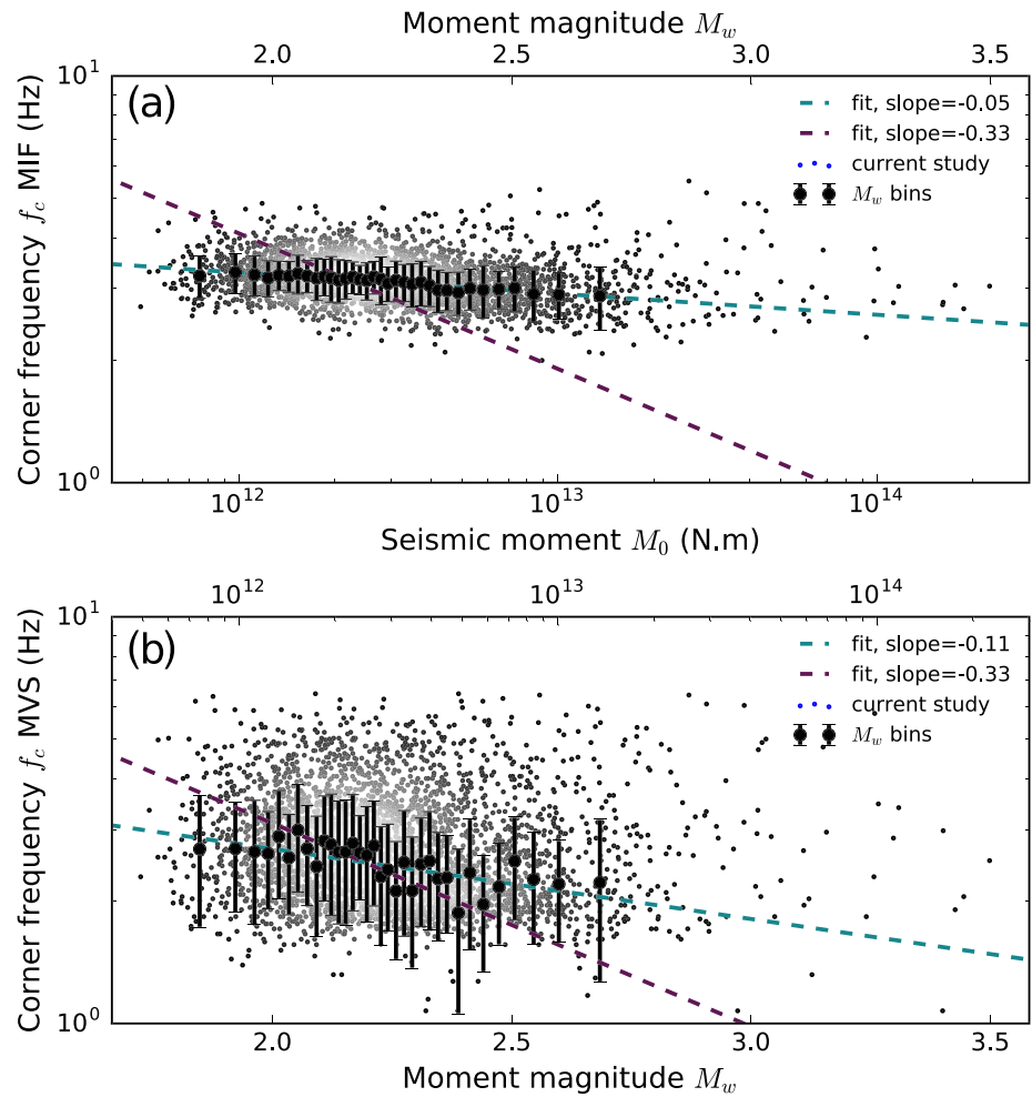
Figure 6. Binned distribution and uncertainties estimation. The measured M_0-f_c is displayed and colored according to point density, for both the mean instantaneous frequency (MIF) and maximum of velocity spectrum (MVS). Seismic moment and corner frequency are binned, and the weighted standard deviation is shown with the error bars (see text for details). Weighted least squares fits to the binned data are displayed, and the fit resulting in the purple scaling has \alpha = \frac{1}{3} as a constraint.
