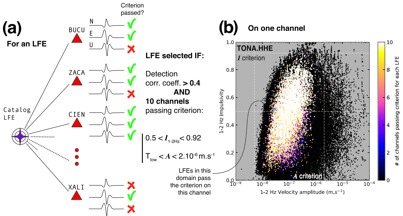
Figure 2. Selection of LFEs. (a) Schematic recapitulation of the selection procedure. (b) Amplitude-impulsivity distribution of all detections recorded on the east component of the station TONA. Each dot is an LFE, and its color corresponds to the number of channels on which it is recorded that pass the criteria. Selected LFEs are white dots: They are recorded on 10 or more channels passing the criterion and fulfill the recurrence and correlation requirements. The amplitude and first impulsivity criteria (Equations 4 and 3) are shown with dashed lines. LFEs in the criterion domain pass the criterion on TONA.HHE, but nine other records passing the criterion on other channels of the network are needed for an LFE to be selected.
