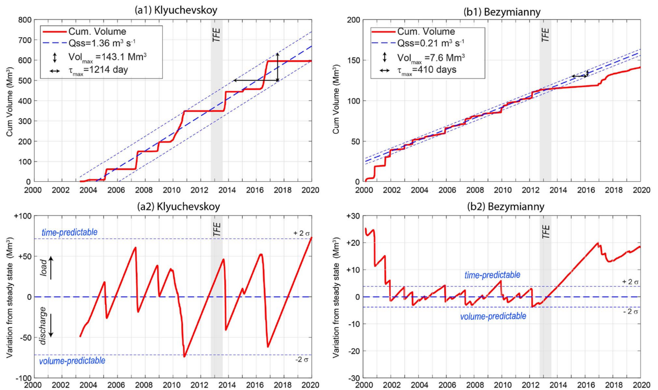
Figure 3. Upper panels. Cumulative volume curves for (a1) Klyuchevskoy and (b1) Bezymianny, derived from satellite measurements (see “Methods”). The linear fits of each cumulative curve represent the linear growth model (blue thick dashed lines) and provide the steady-state output rate ( Q_{ss} ). The two parallel lines (linear model \pm 2\sigma ) define the maximum eruptible volume ( Vol_{max} ) and the maximum response time ( \tau_{max} ) for the inferred steady-state condition. Lower panels. Load and discharge model for (a2) Klyuchevskoy and (b2) Bezymianny. The variation from the steady-state is calculated as the residual between the linear growth model and the observed cumulative volume curves. A two-fold standard deviation ( \pm 2\sigma ) of residual is used to define the upper and lower volume limits for the load-discharge model. In this plot, a time-predictable system would have a near-constant upper threshold of the volume load when eruptions occur. A volume-predictable system would have a near-constant lower threshold. An entirely predictable system would have both. The gray bar indicates the timing of the 2012 Tolbachik Fissure Eruption (TFE). Time series generated using MATLAB software ( www.mathworks.com ).
