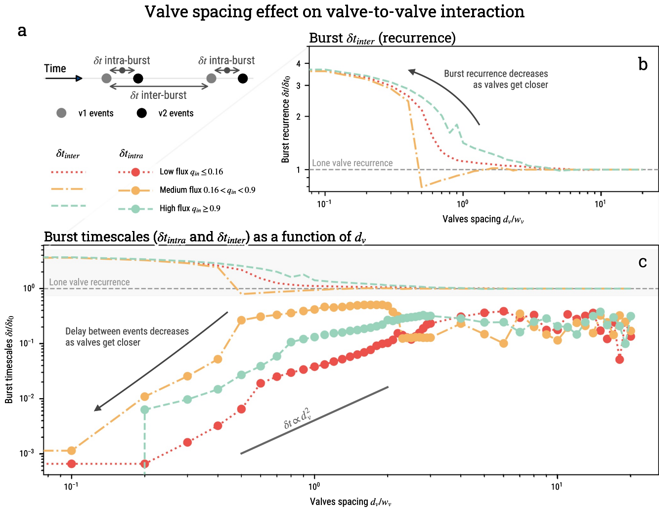
Figure 5. Effect of valve spacing on valve-to-valve interaction. (a) Two timescales describe a two-event burst: \delta t_{intra} is the delay between events in the burst, and \delta t_{inter} is the recurrence delay of the burst. In panels (b) and (c), we observe how \delta t_{inter} (no markers on the line) and \delta t_{intra} (circle markers) evolve as a function of valve spacing for low (red, dotted line), intermediate (yellow, dash-dot line) and high (green, dashed line) flux values. Both timescales are normalized by \delta t_0 , the period of activation of a valve subjected to the same flux. For sufficiently large valve spacing ( d_v > 5w_v ), valves do not interact and act as isolated valves. As valves get closer, events get closer, and the bursts are less frequent.
